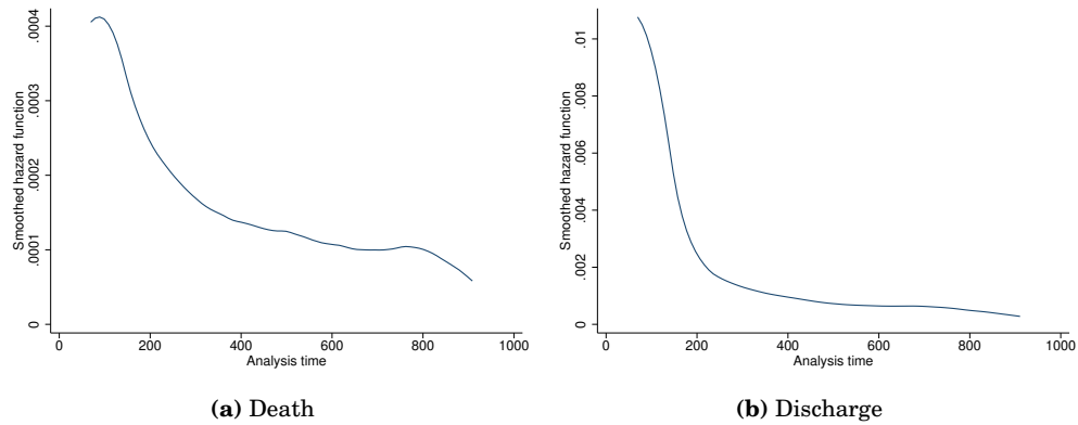
Figure A.21. Cause-Specific Baseline Hazard Functions, h_{c,0}(t)
