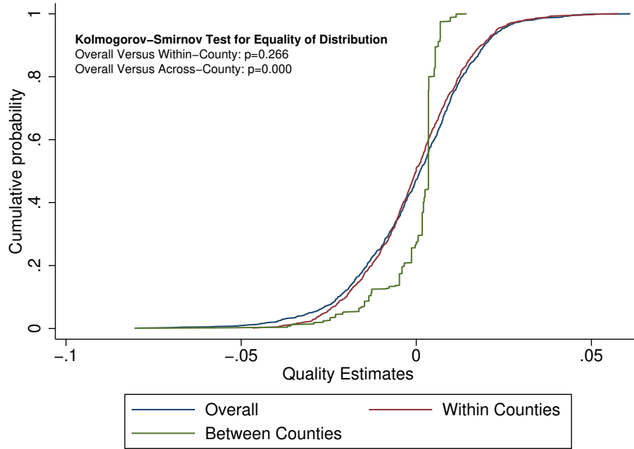
Figure II. ECDF of Empirical Bayes Quality Estimates
